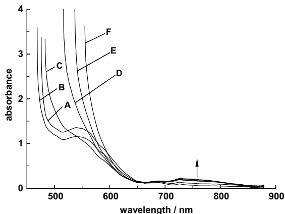
Fig. 3. Reaction of \text{MoCl}_6^{3-} and Mo with \text{Cl}_2 in \text{LiCl-KCl} ( 400^\circ\text{C} ). Time of reaction, min: A, 0; B, 1; C, 4; D, 6; E, 8 and F, 11.
