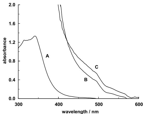
Fig. 5. Reaction of \text{MoO}_2 with \text{Cl}_2 in \text{NaCl-KCl} melt at 700^\circ\text{C} . A, \text{MoO}_2 in \text{NaCl-KCl} melt for 3 min under Ar atmosphere containing trace amounts of chlorine. B, 3 min chlorination. C, total of 44 min chlorination.
